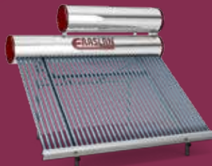
36 Tüplü Krom Double 36 Tubes Inox Cover Double
